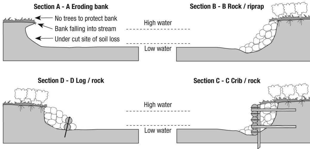
Figure 20. Conceptual drawings of several types of stream bank stabilization techniques.
